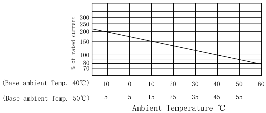
Compensation Curve
